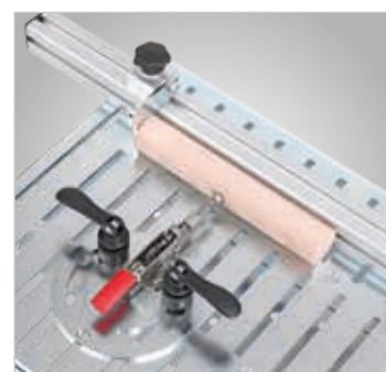
Adapter plate with clamp, horizontal
