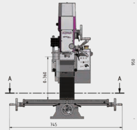
Dimensions MH 22V
