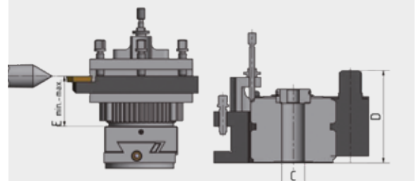
Tool holder head dimensions
